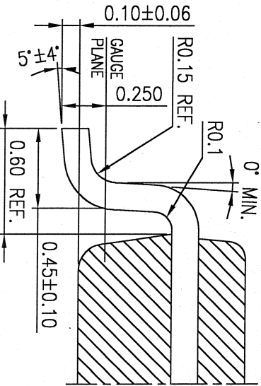
DETAIL "A" (S=32:1)
