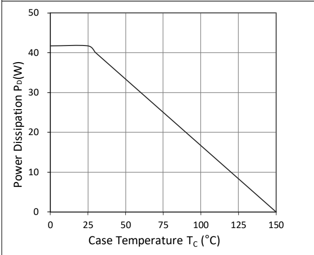
Figure 9. Power Dissipation
