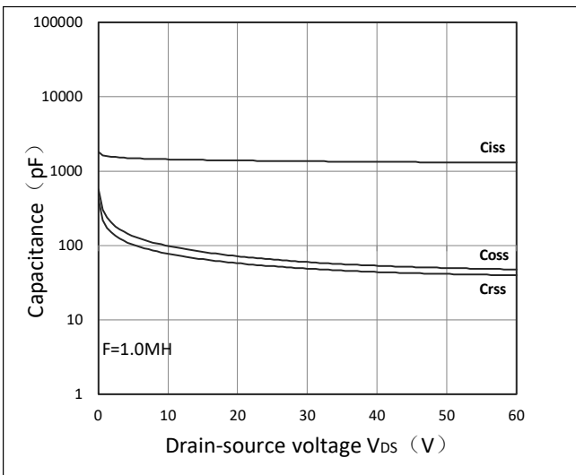
Figure 7. Capacitance Characteristics
