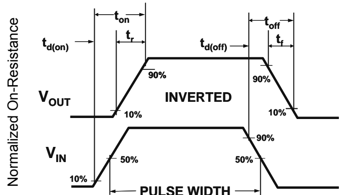
Figure 2: Switching Waveforms
